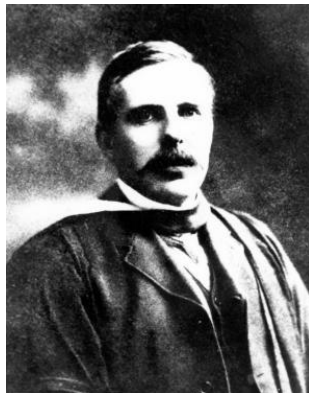
Ernest Rutherford (1871-1937).
